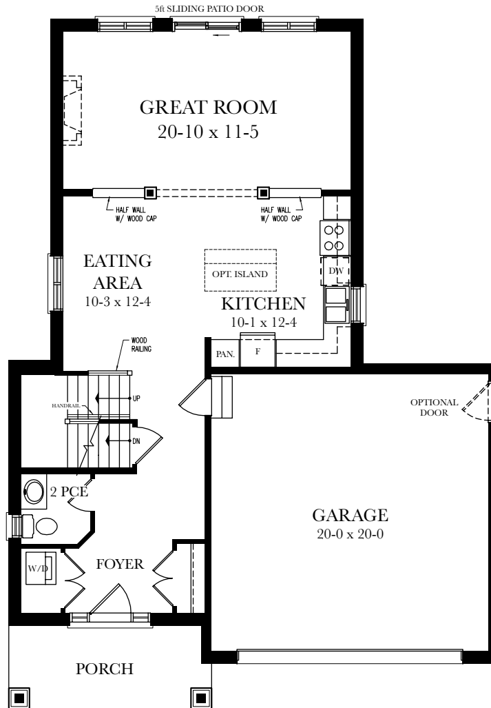
MAIN FLOOR PLAN ELEVATION A 851 SQ.FT
