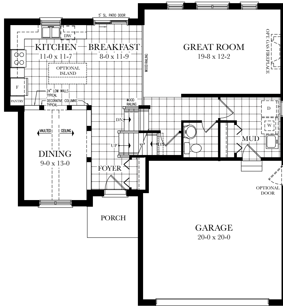
MAIN LEVEL PLAN - 983 sq.ft.
