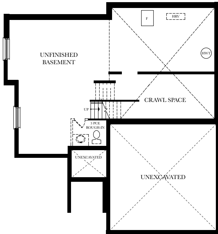
BASEMENT PLAN
