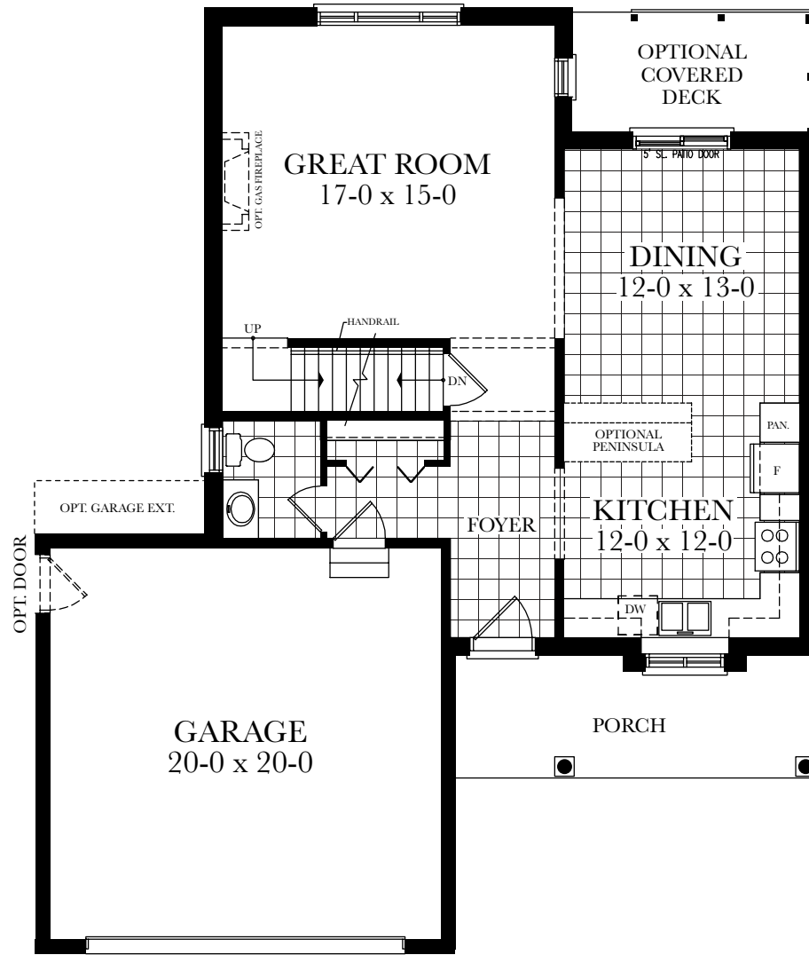
MAIN FLOOR PLAN - 893 sq.ft.
